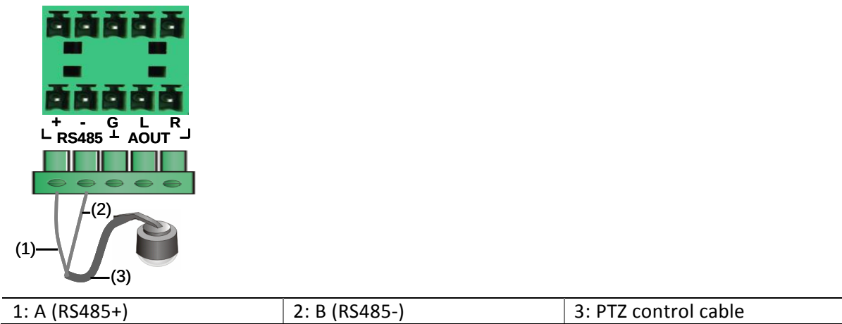
Figure 2-8 Connect a type A phoenix connector to a PTZ control cable
