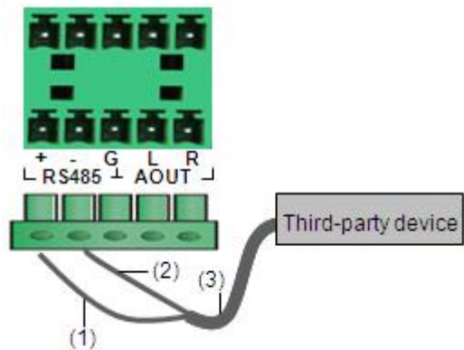
Figure 2-18 Connect a type A phoenix connector to a third-party device
