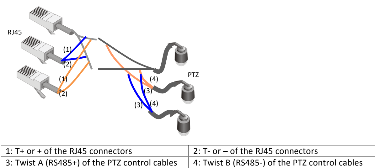
Figure 2-7 Connect multiple RJ45 connectors to multiple PTZ control cables (zigzag-shape)
