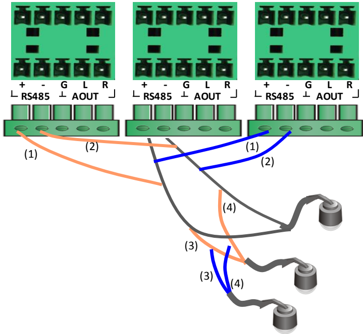
Figure 2-15 Connect multiple phoenix connectors to multiple PTZ control cables (zigzag-shape)
