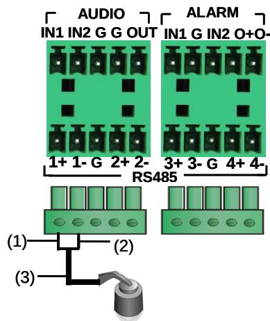
Figure 2-9 Connect a type B phoenix connector to a PTZ control cable
